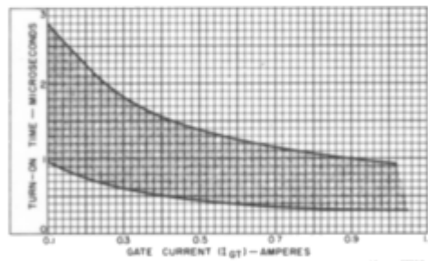
Fig. 12 - Turn-on time characteristics.
