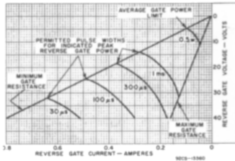
Fig. 11 - Reverse gate characteristics.
