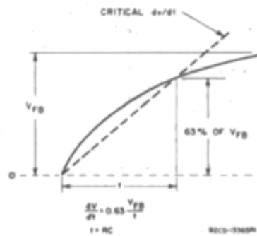
Fig. 1—Waveshape of critical dv/dt rating test.
