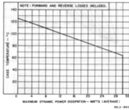
Fig. 4—Maximum average total power dissipation as a function of case temperature.
