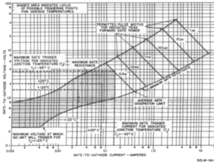
Fig. 10 - Forward gate characteristics.
